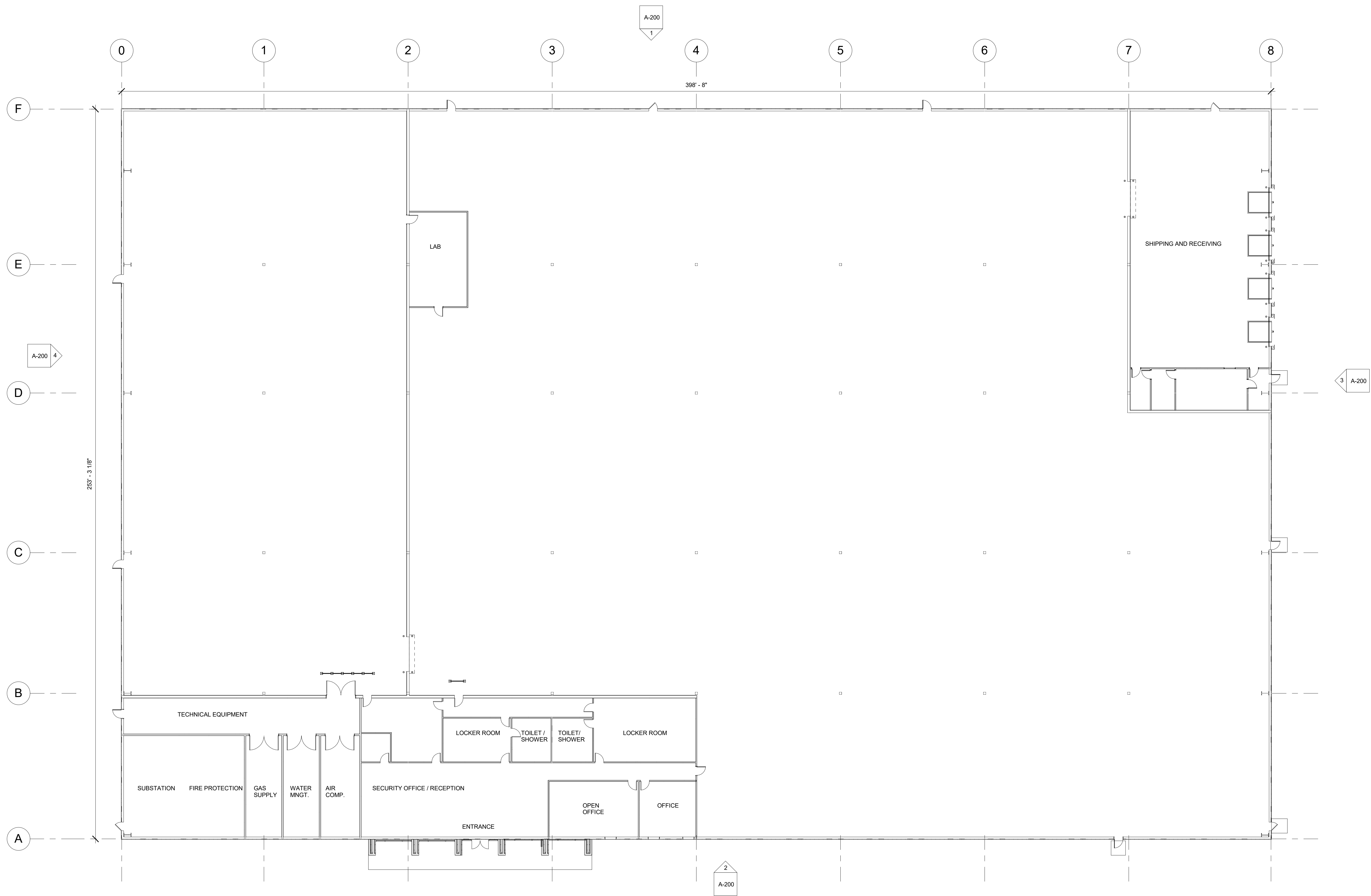
1 OVERALL NEW FLOOR PLAN 1/16" = 1'-0"
